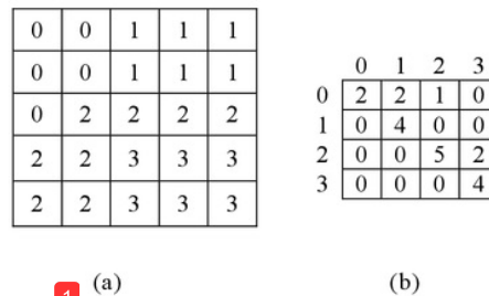
Fig. 6 (a) Example of an image with 4 gray level image. (b) GLCM for distance 1 and direction 0^\circ
