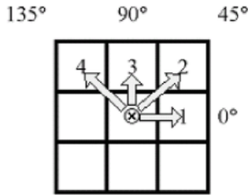
Fig. 7. Direction of GLCM generation. From the center (⊗) to the pixel 1 representing direction = 0° with distance d = 1, to the pixel 2 direction = 45° with distance d = 1, to the pixel 3 direction = 90° with distance d = 1, and to the pixel 4 direction = 135° with distance d = 1.
